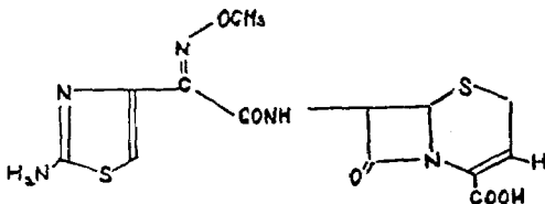
Fig. 1. Chemical structure of the ceftizoxime.
