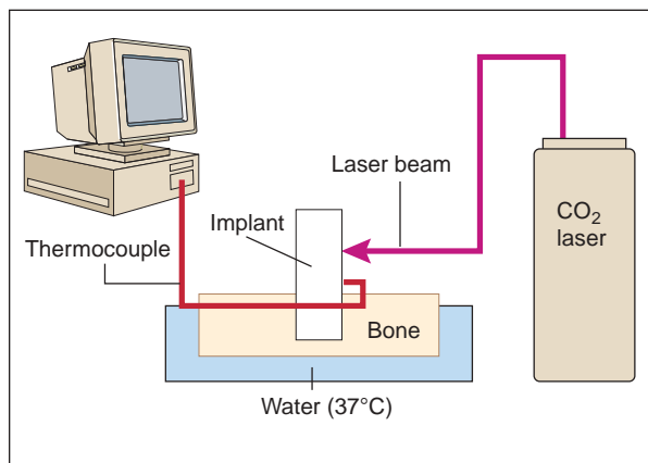
Fig 1 Experimental setup in vitro. The implant-bearing bone was fixed in a water bath, assuring that the level of immersion could not reach the marginal rim of the bone with the thermocouple in the implant-bone interface.
